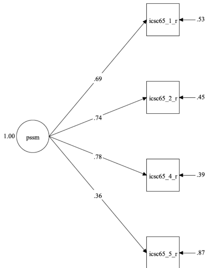
Figure 4 Standardised factor loadings for the PSSM, K cohort, wave 9
