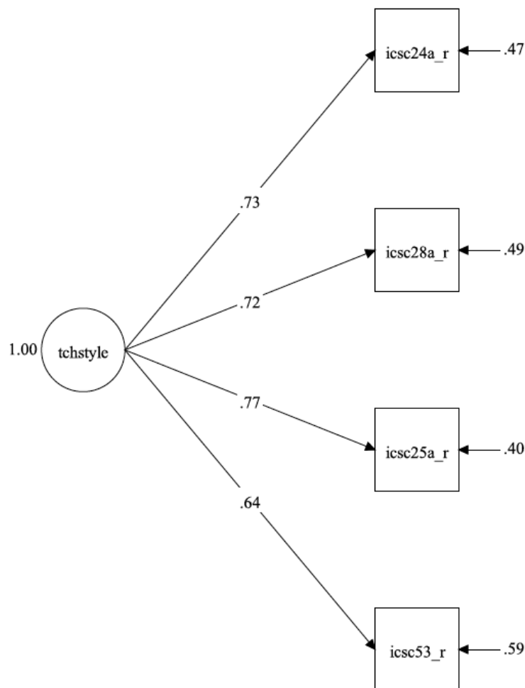
Figure 7 Standardised factor loadings for teacher style, K cohort, wave 9
