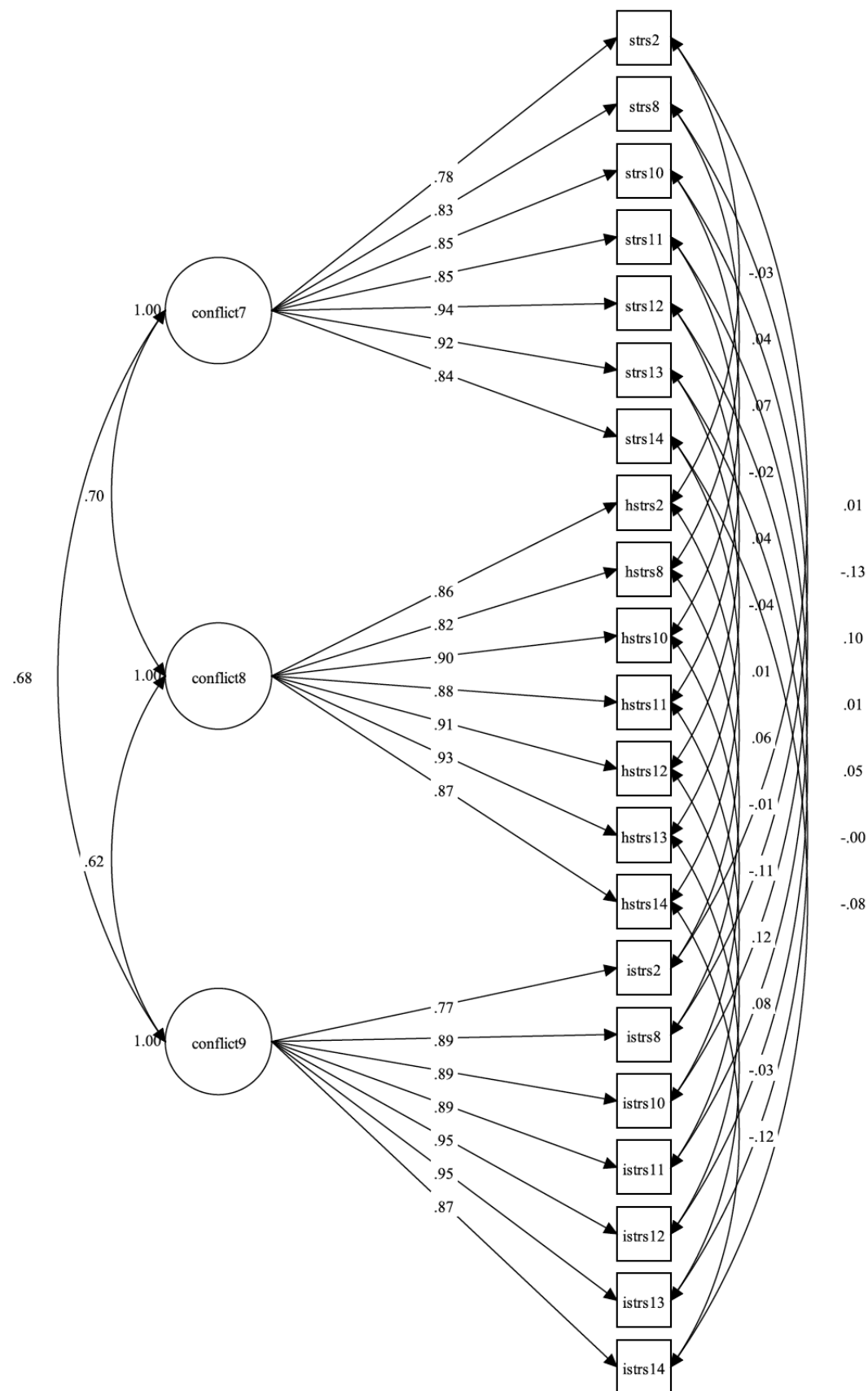
Figure 15 Factor loadings on conflict for the STRS, B-cohort, waves 7–9
